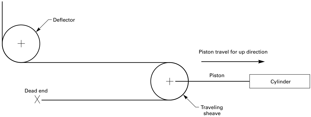
Figure B-1 Pusher-Type Roped-Hydraulic Elevators
