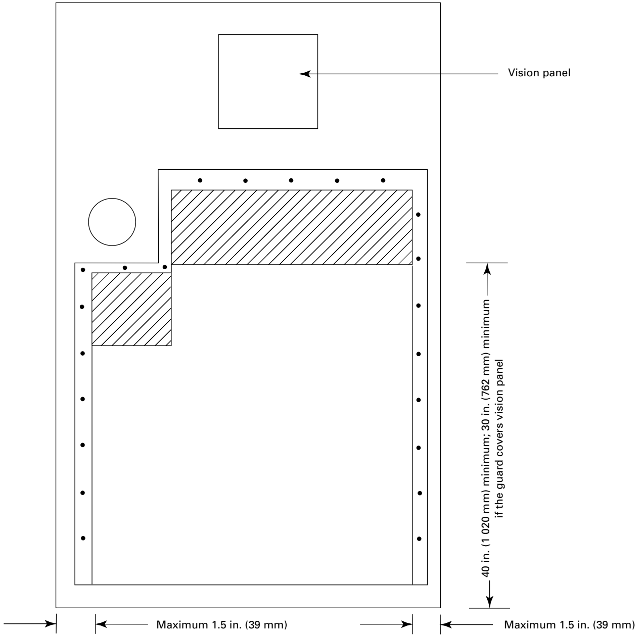
Figure A-5 Typical Space Guard for Swinging Doors With Cutout for Doorknob, Handle, or Pull Bar
