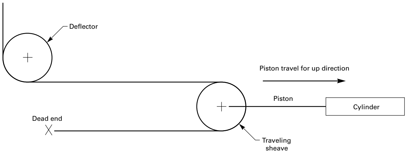
Figure B-2 Puller-Type Roped-Hydraulic Elevators
