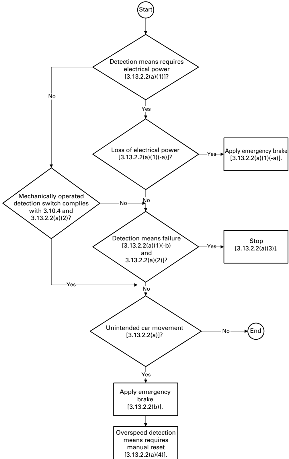
Figure E-2 Unintended Car Movement Protection
