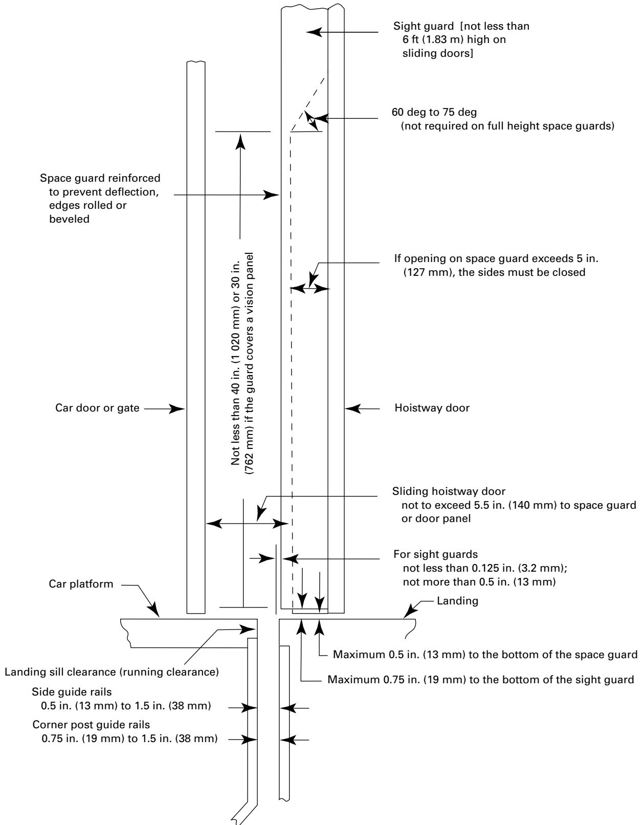
Figure A-3 Typical Sliding Hoistway Door Space Guard and Sight Guard
