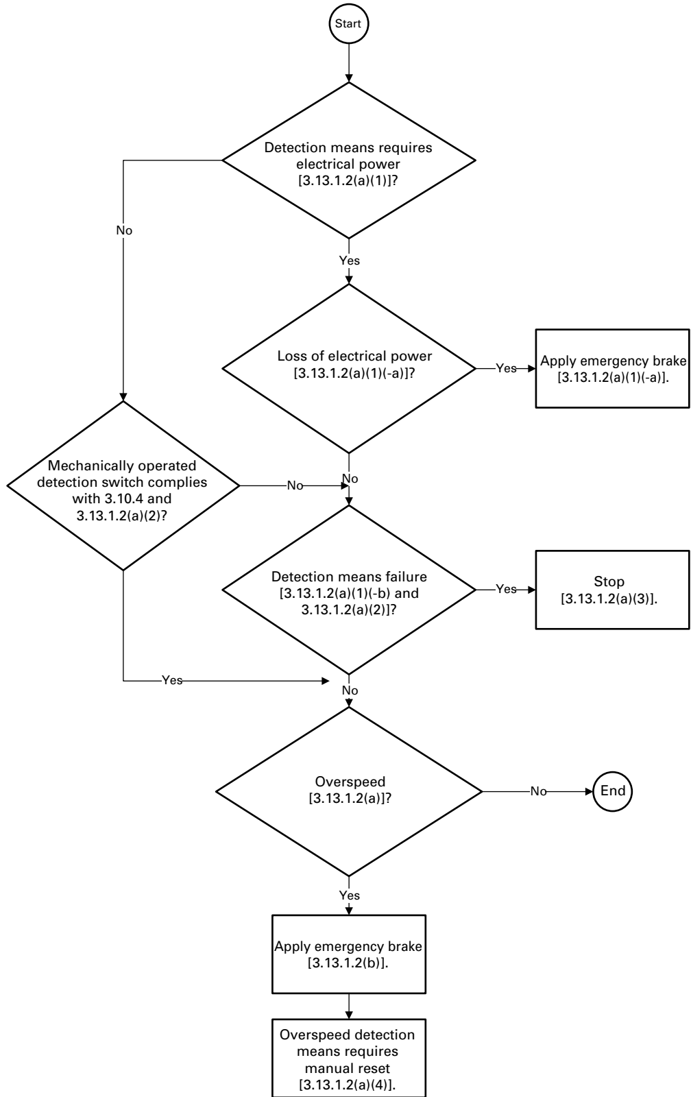
Figure E-1 Ascending Car Overspeed Protection
