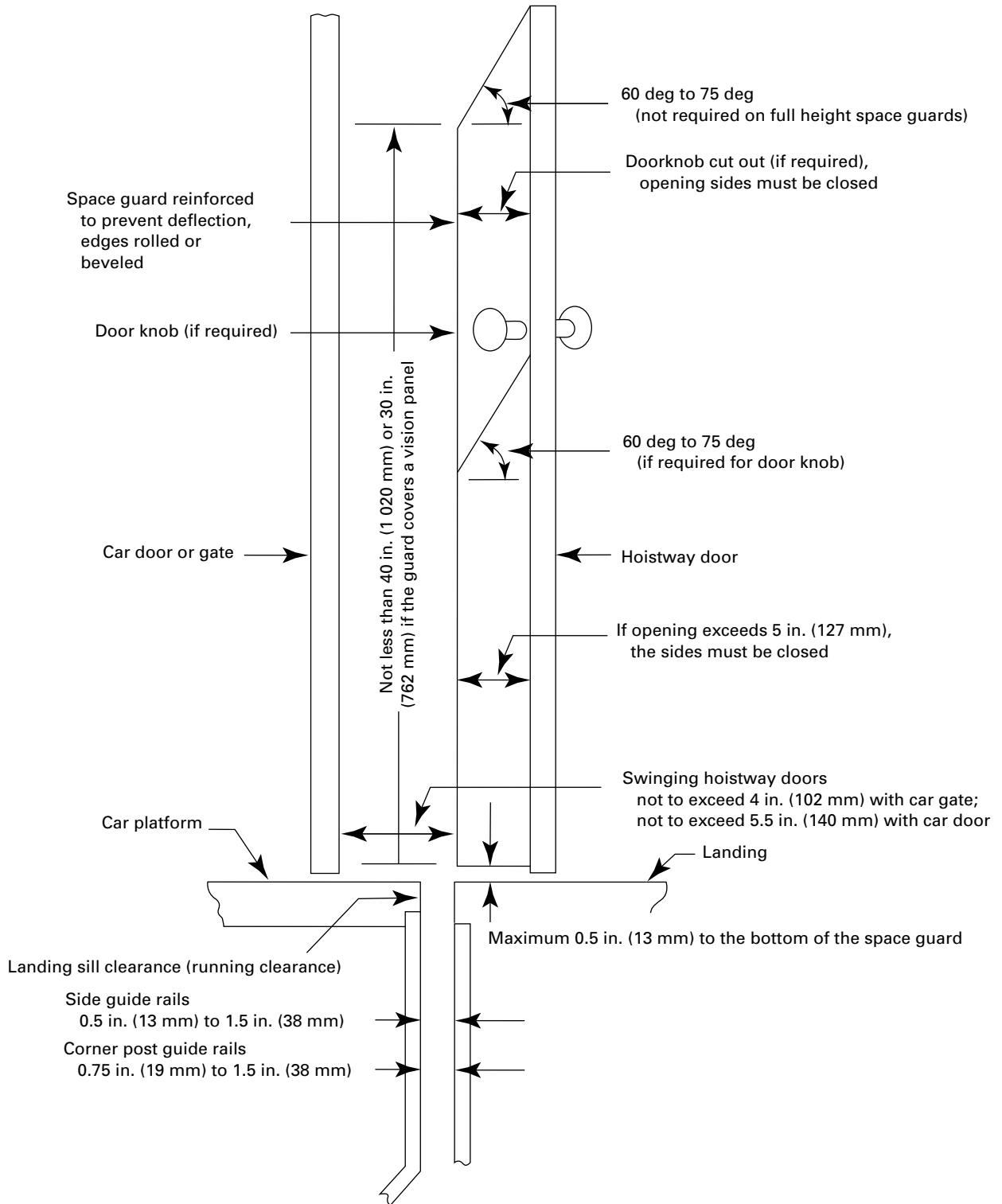
Figure A-4 Typical Swinging Hoistway Door Space Guards
