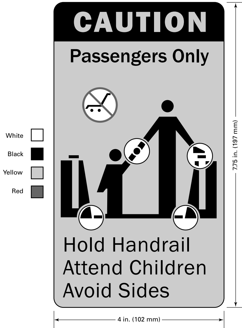
Figure 5.3.11-1 Caution Sign
